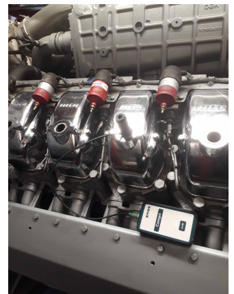
Compri installed on a power plant MTU 4000 (Powertec 1160) 4-stroke gas engine
